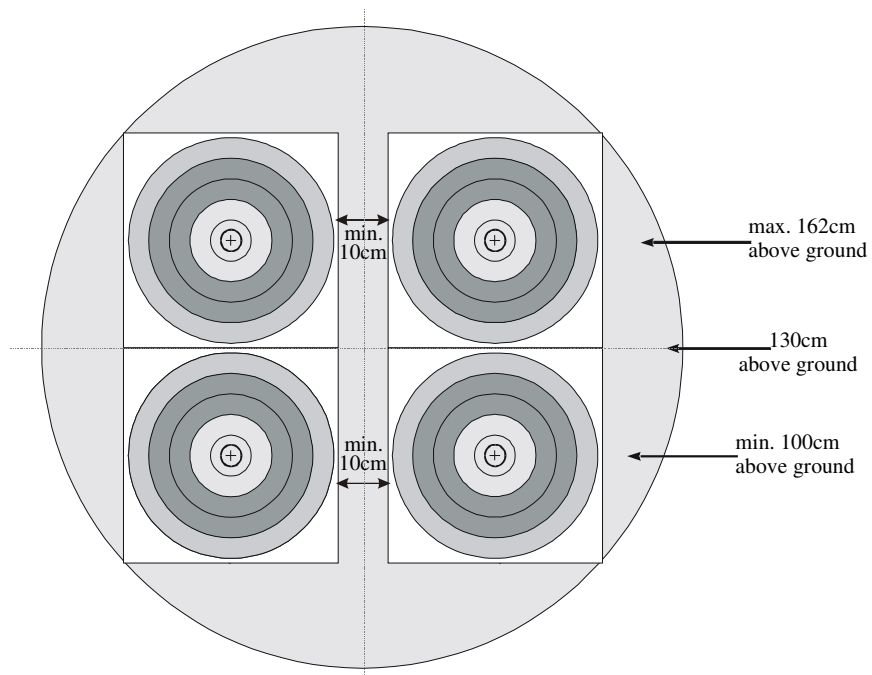
80cm-center four-center-set-up 80cm-Zentren 4 Zentren
